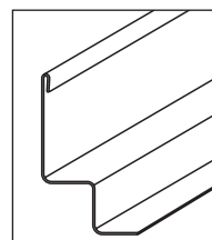
Wand W-profiel Fe/Alu 0.8 mm (45 x 21 x 21 x 18.5)
