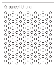
Ø 1 mm ⇄ 2 ⇄ 3.46 Openheid 23%
