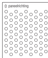
Ø 1.5 mm ⇄ 3 ⇄ 5.2 Openheid 23%
