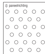
Ø 2 mm ⇄ 8.66 ⇄ 5 Openheid 16%
