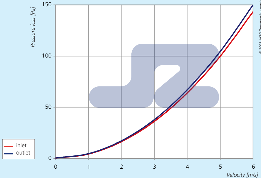
Graph pressure loss
