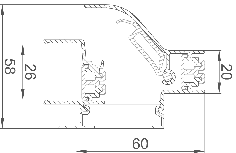
Smart 60 / 26
