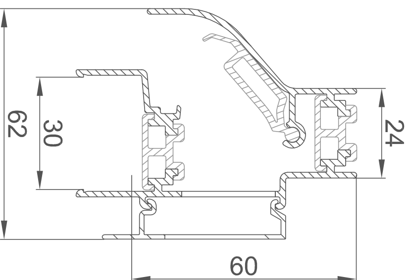
Smart 60 / 30
