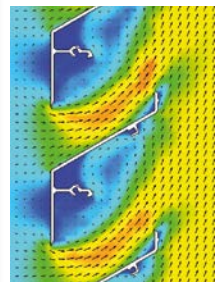
Lamelstep 75 IN
