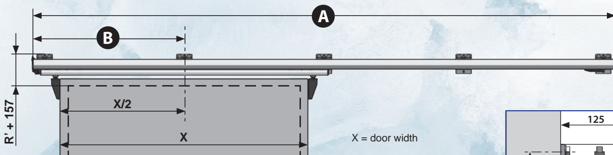
Automatic Kit 5010 for 3530 / 7530 with motor 370W
