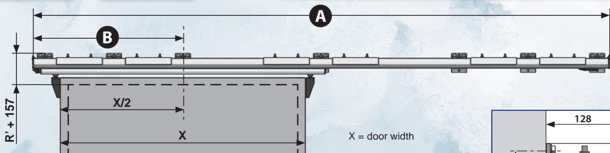
Automatic Kit 5000 for 3530 -300Kg / 7530-300Kg with motor 550W
